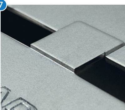
SEMI-CORTE MICRO-UNION
